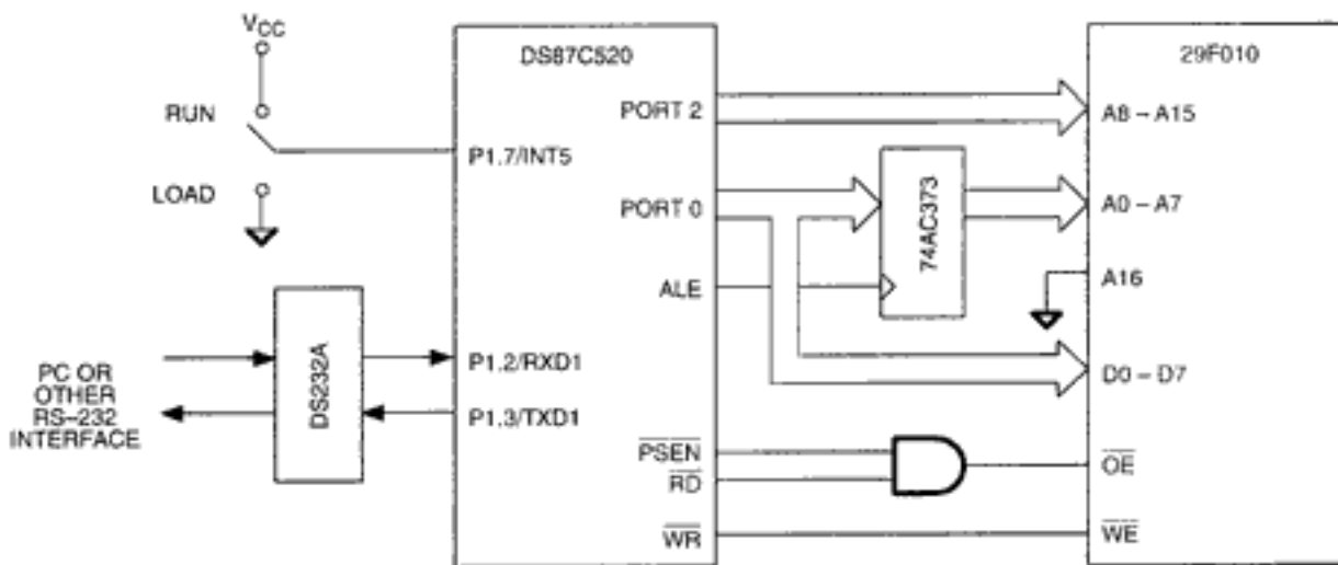
Figure 2. Bootloader Hardware
