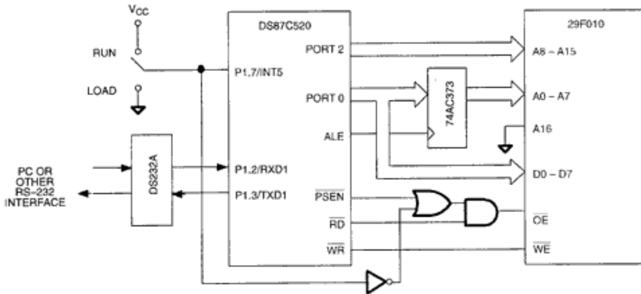
Figure 3. Bootloader Hardware for DS87C520/DS87C530 Revision A4
